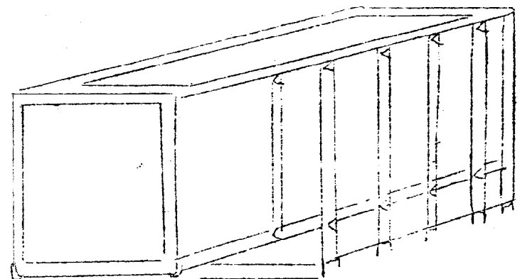
Frame Made from 1/8" Angle and 1/4" Channel Iron
