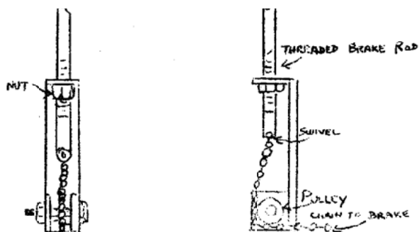
DETAIL A BRAKE ROD BRACKET
