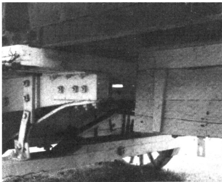
Rear Undergear and Possum Belly [W. Bahr Photo]
