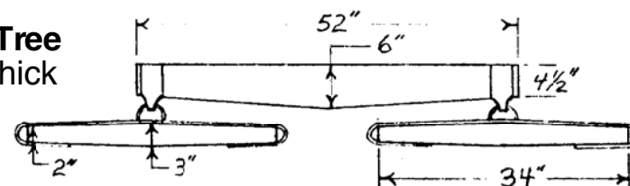
Hagenbeck-Wallace Baggage Wagon No. 70
