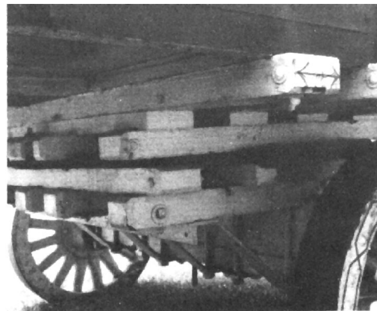
Front Undergear -Fifth Wheel from Rear [W. Bahr Photo]
