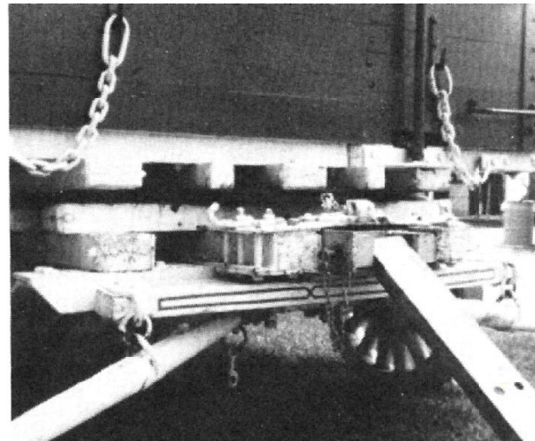
Front Undergear - Tongue [W. Bahr Photo]
