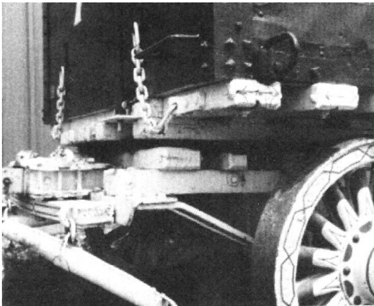
Front Undergear - Left View [W. Bahr Photo]
