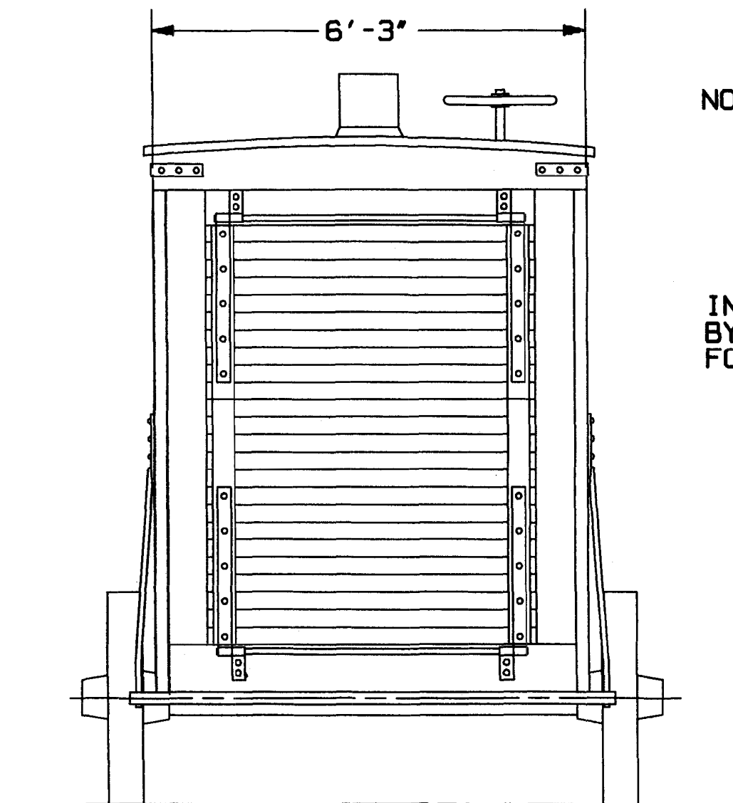
REAR VIEW
