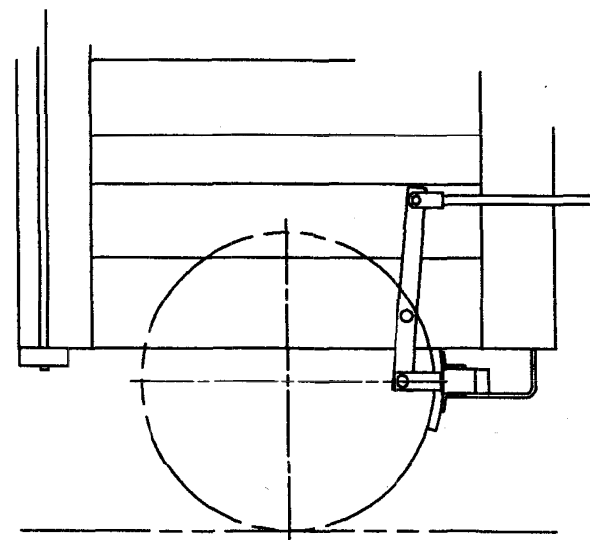
BRAKE LEVER SYSTEM
