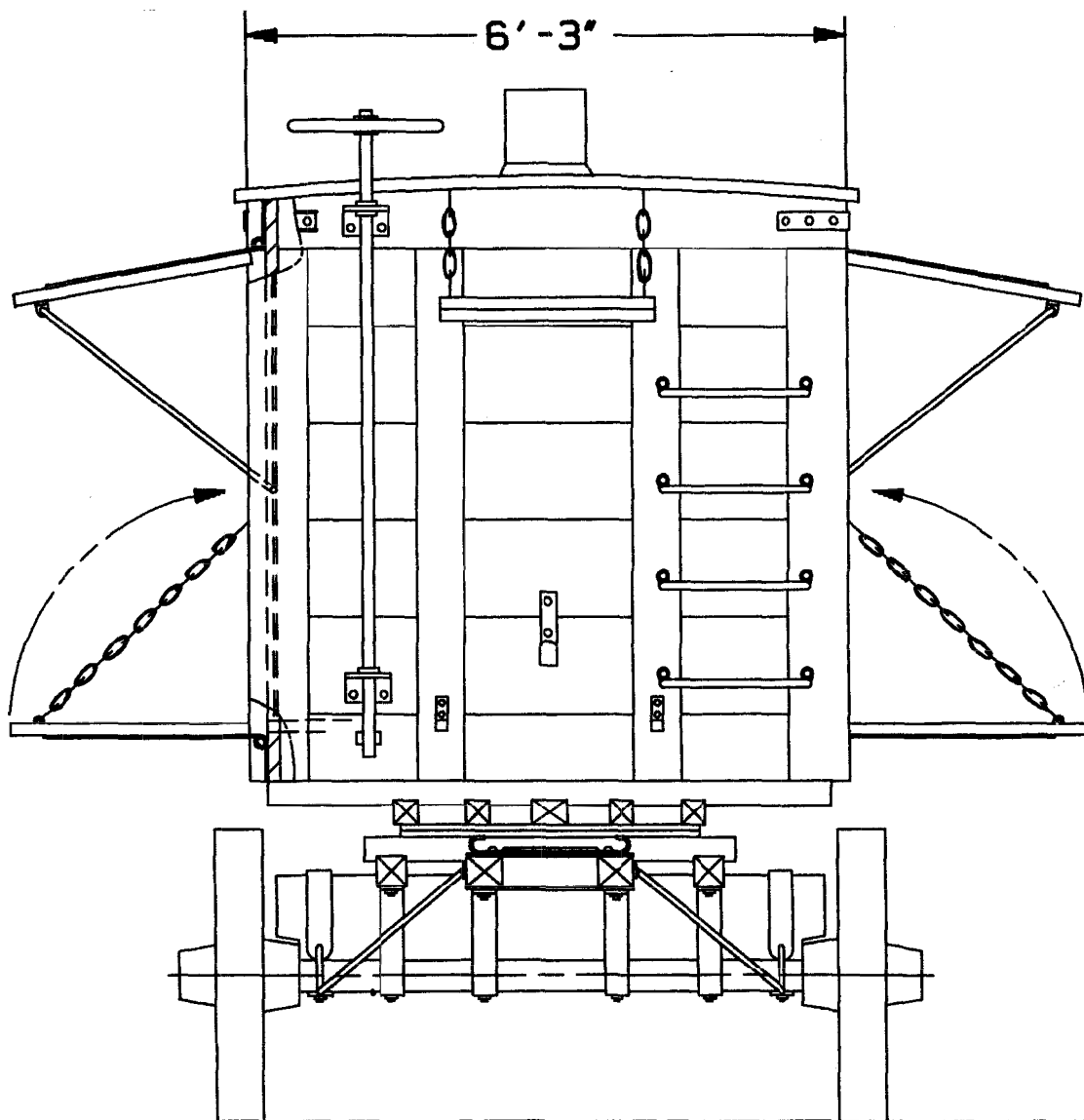
FRONT VIEW
