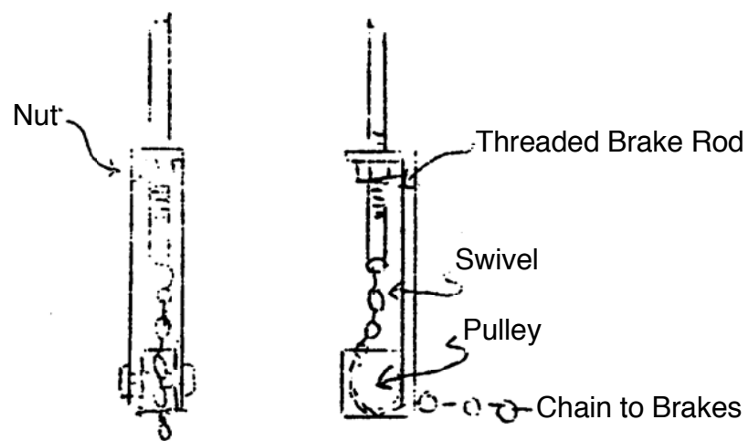
Detail "A" - Brake Rod Bracket
