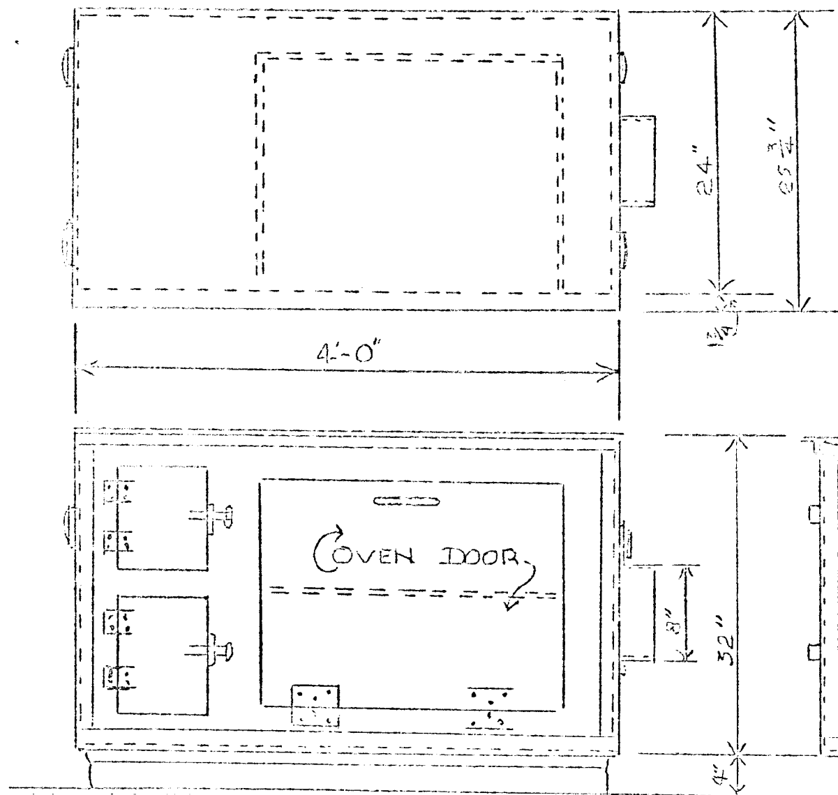
Front View
