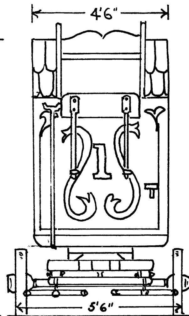
FRONT ELEVATION
