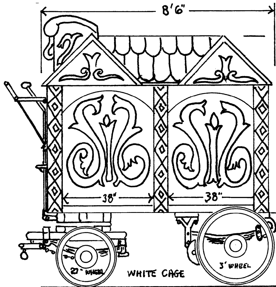
SIDE ELEVATION
