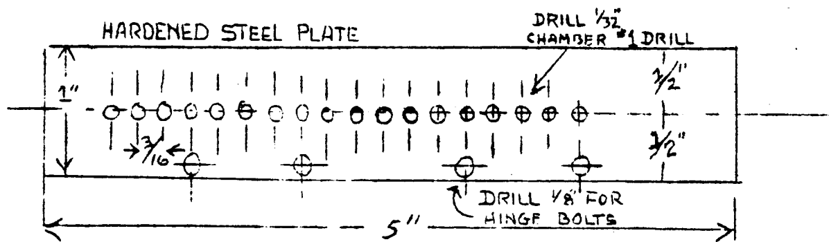
DRILL JIG - TOP VIEW
