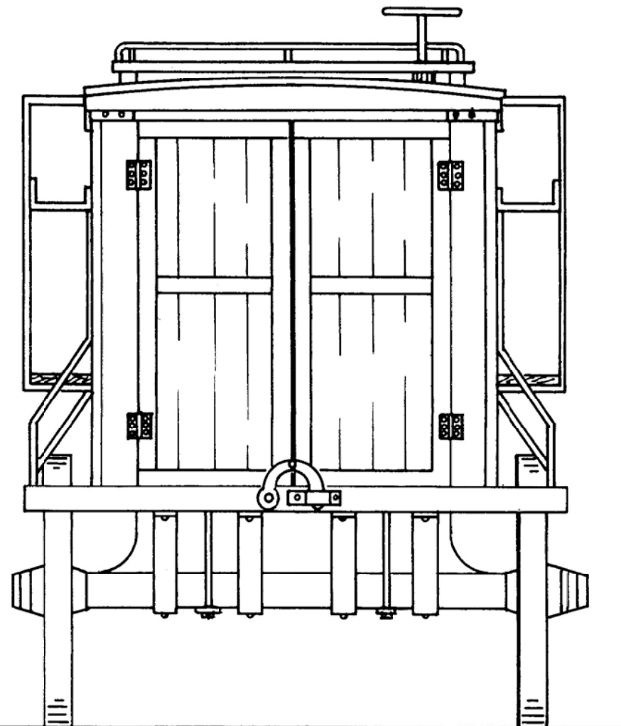
back view
