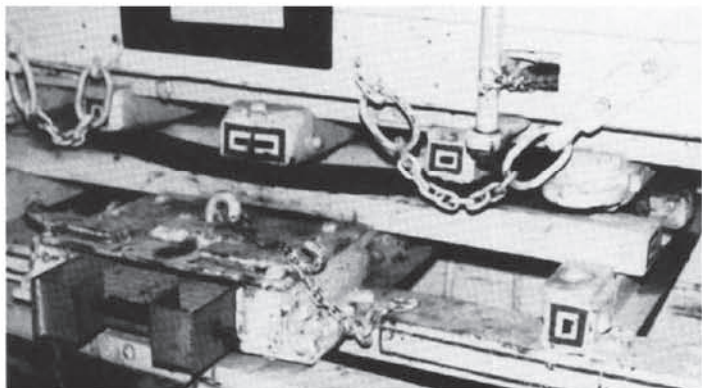
Fifth Wheel - Front View - Close-up
