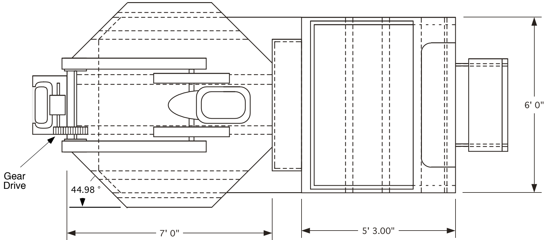
Top View
