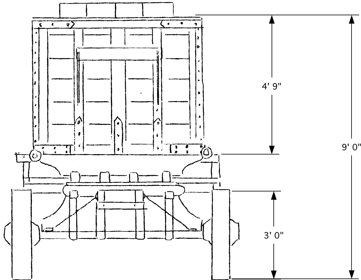
Front View
