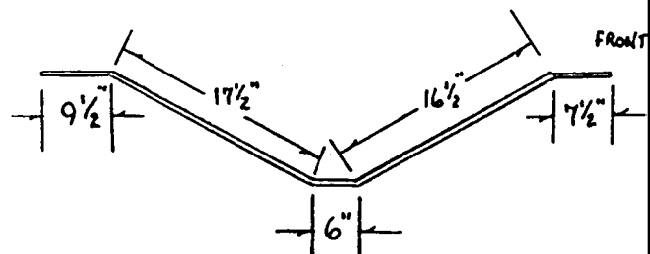
2 1/2" WIDE STEEL STRAP (OUTER)
