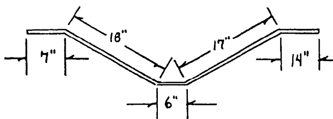
3" WIDE STEEL STRAP (INNER)
