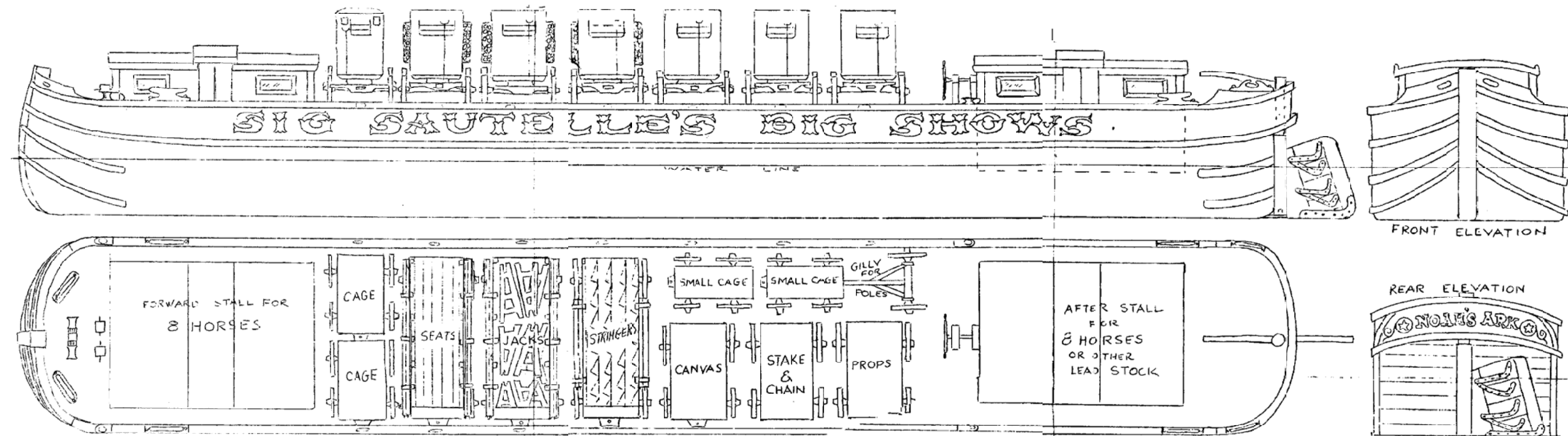
Canal Boat for Carrying Horses and Show Equipment
