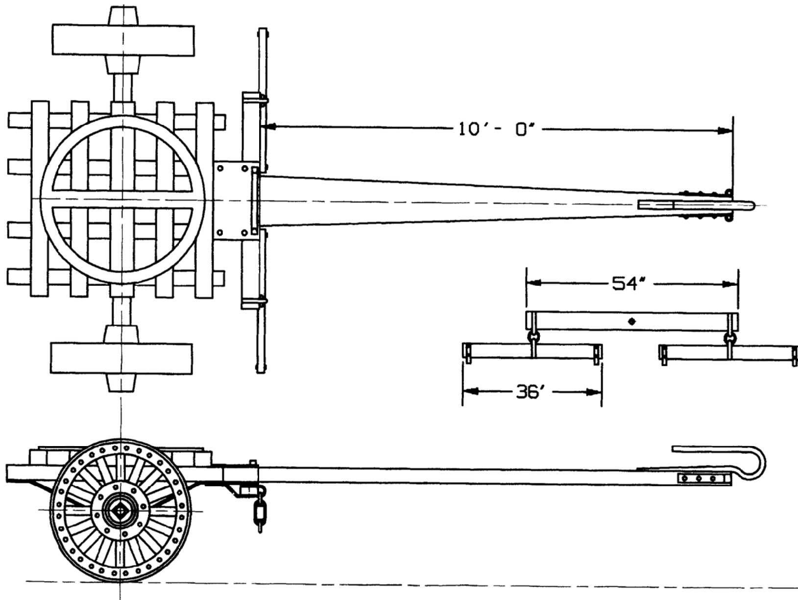
Front Undergear
