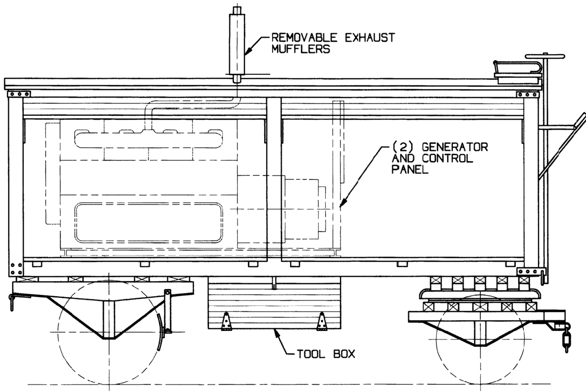
Interior View
