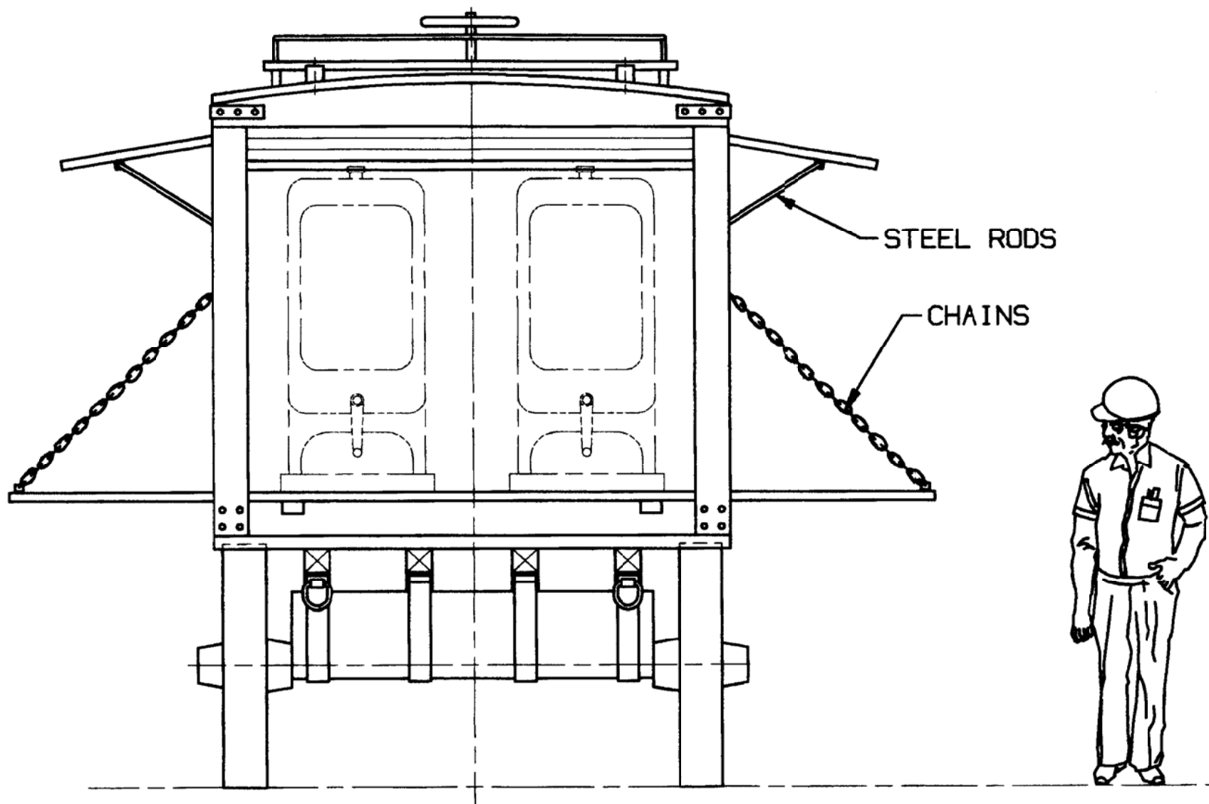
Rear View
