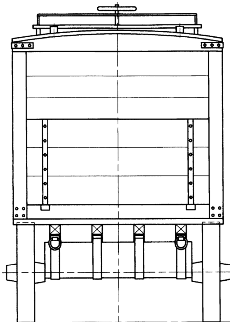
Rear View
