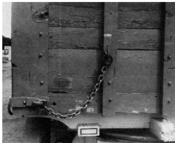
Photo No. 10 – Front view of corner construction
