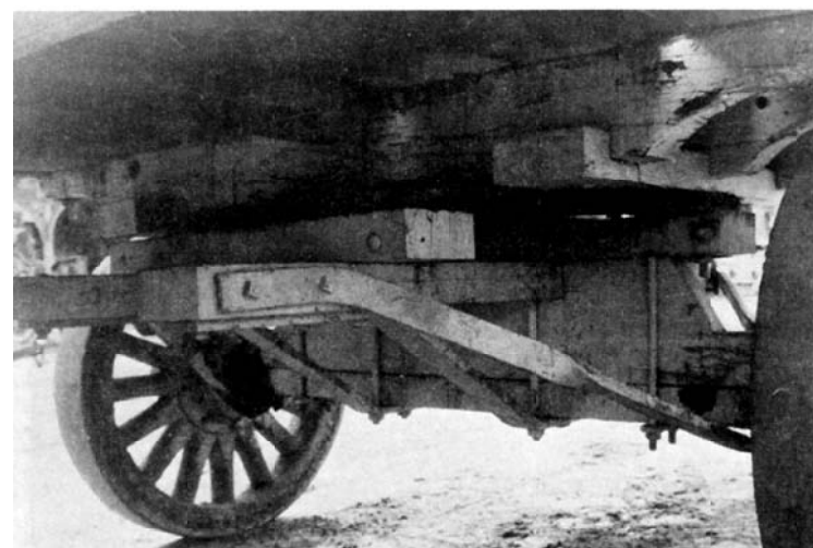
Photo No. 4 – Rear view of front undergear
