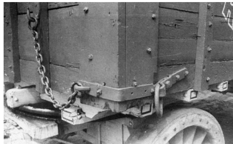
Photo No. 9 – Corner bracket, chain and rims construction
