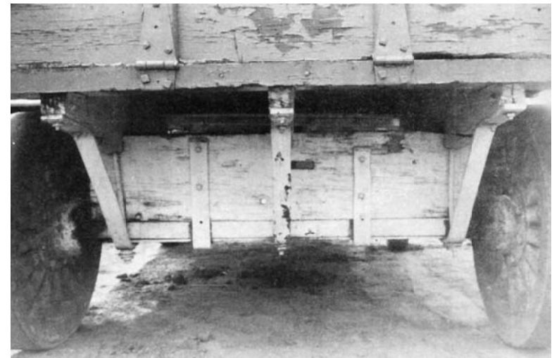
Photo No. 14 – Front view of rear undergear
